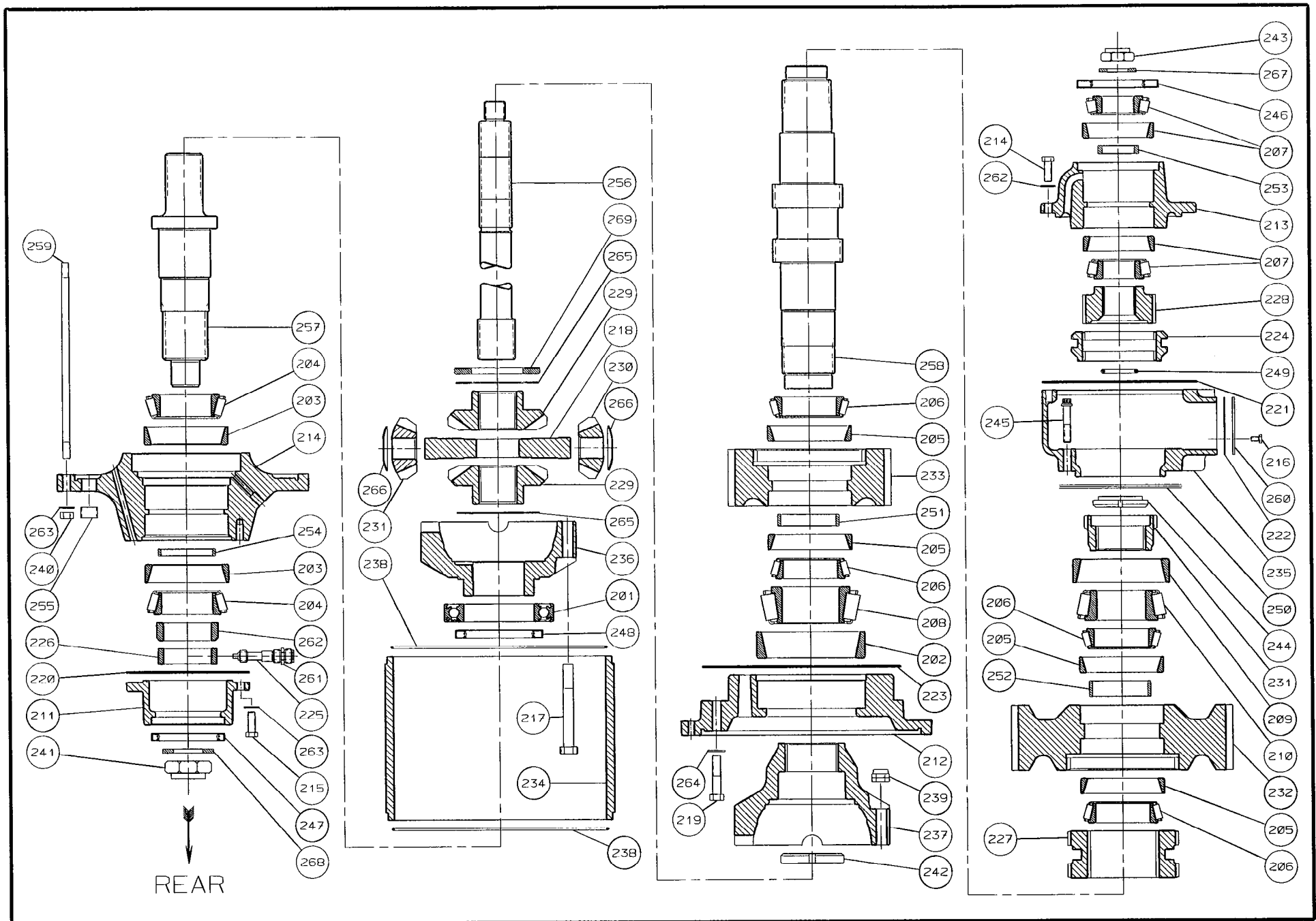
FIGURE 8.1 , TC-142PD 50/50 , LOWER SHAFT PARTS
